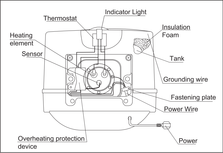
Schematic Construction
